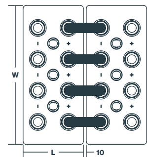
19 OPzS-ET3300SOLAR - 26 OPzS-ET4550SOLAR
