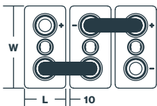
2 OPzS-ET160SOLAR - 7 OPzS-ET1070SOLAR
